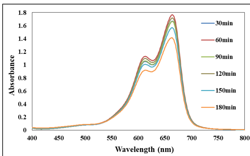
Fig.3 UV-vis spectrum showing degradation of MB solution under UV light irradiation
