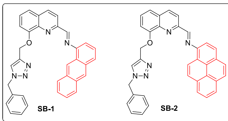
Figure 1. Synthesized Schiff bases
