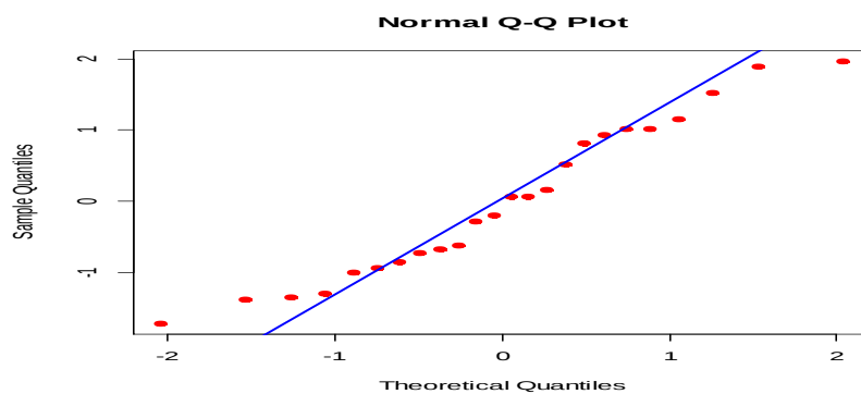
Figure 3: Quantile to quantile plot
