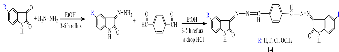
Scheme 1. Synthesis
